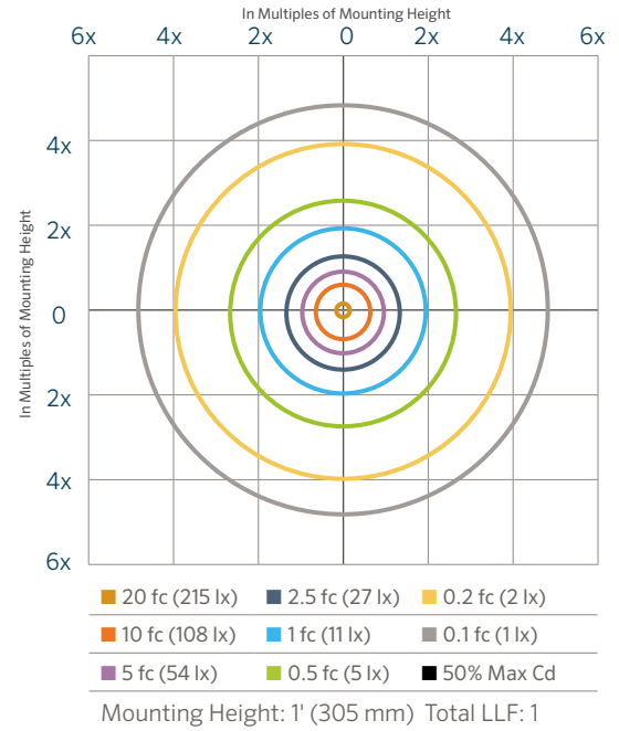
aEmpress-18 ZDC Isofootcandle Plot
