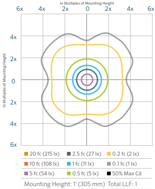
aEmpress-18 1LED Isofootcandle Plot
