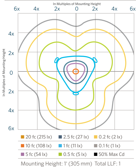
aEmpress-18 3LEDT Isofootcandle Plot
