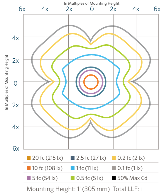
aEmpress-18 3LED Isofootcandle Plot
